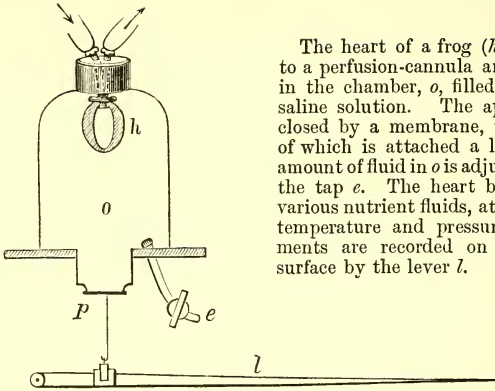
FIG. 13.—Roy's heart-tonometer.
